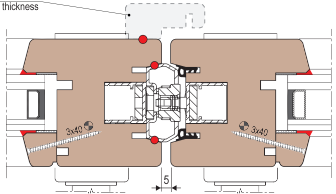
COAXIAL SASHES CENTRAL POINT (with hooks lock)
