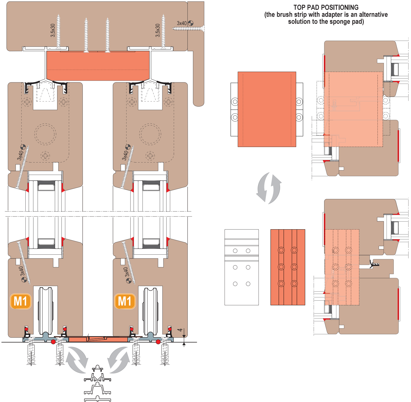
XC S-LINE CARRIAGES (SEAT 16 mm)
