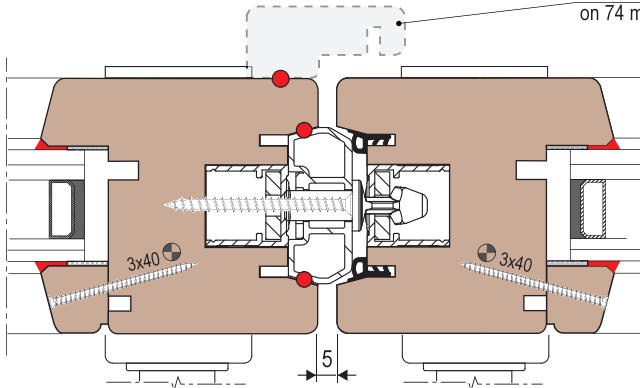
COAXIAL SASHES CENTRAL POINT (with pins lock)
