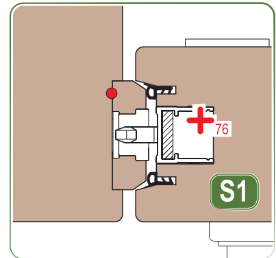
COAXIAL SASHES CENTRAL POINT (with hooks lock)
