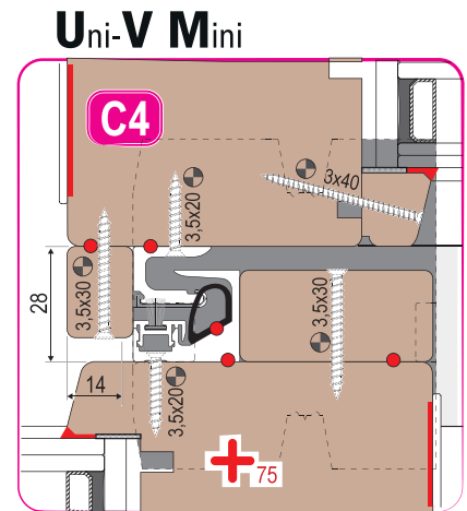
Position the pad as indicated
