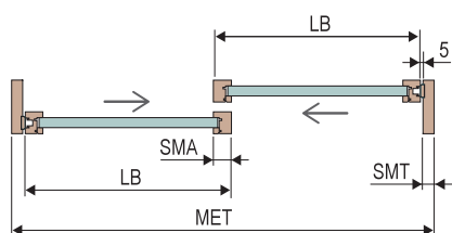
Layout B 2 sliding sashes LB=[MET-2x(SMT+5)]:2+SMA:2
