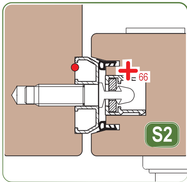
COAXIAL SASHES CENTRAL POINT (with pins lock)
