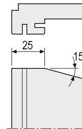
Shaping of sliding sash listel (only for layout B and F)
