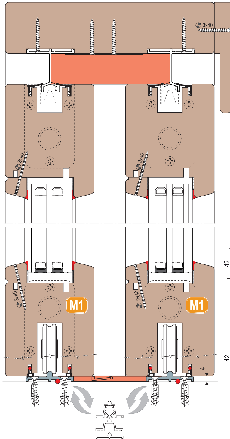
XC S-LINE CARRIAGES (SEAT 16 mm)
