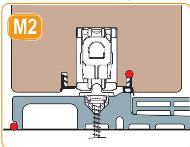
XC S-LINE CARRIAGES (SEAT 22 mm)
