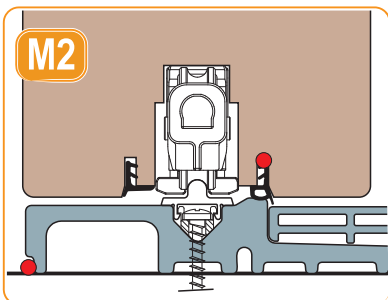
XC S-LINE CARRIAGES (SEAT 18 mm)
