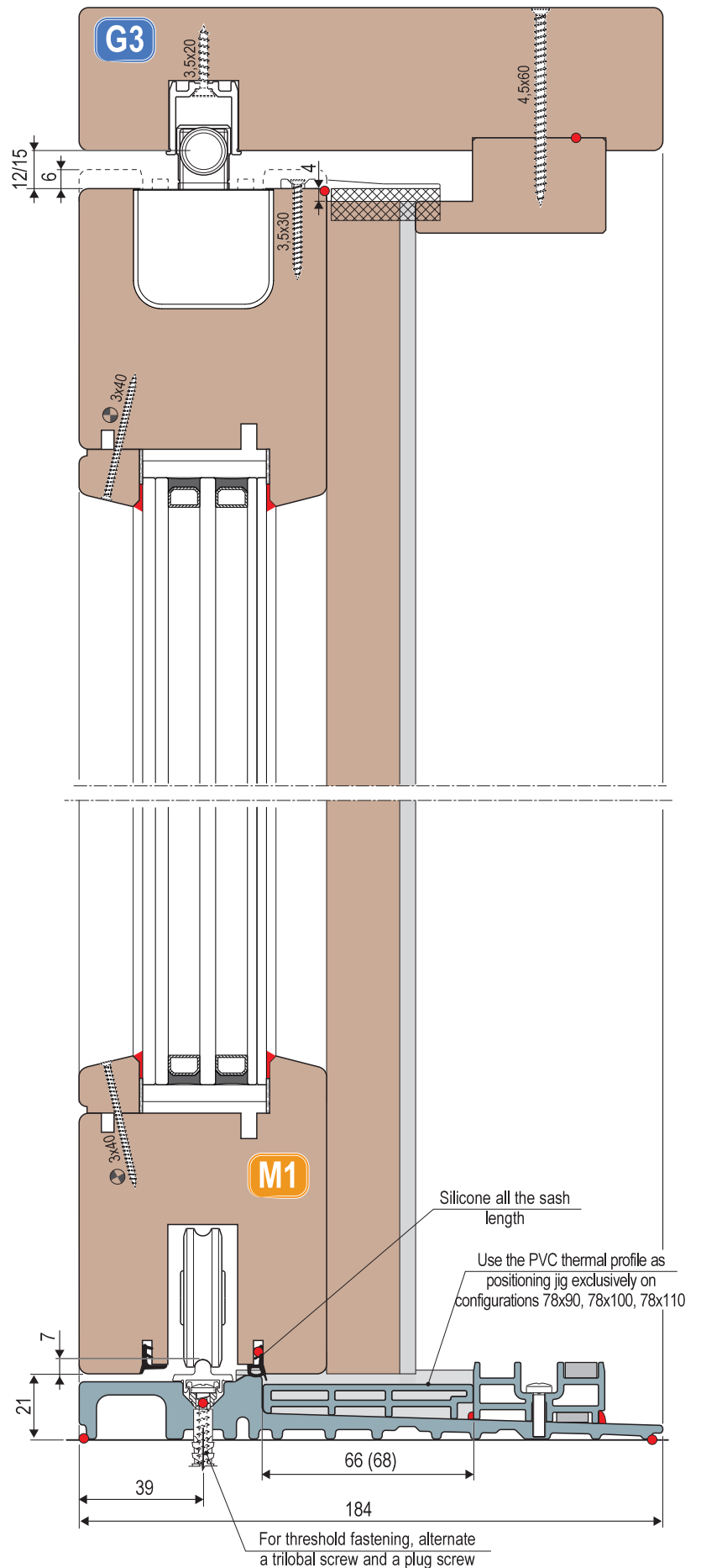
XC S-LINE CARRIAGES (SEAT 22 mm)
