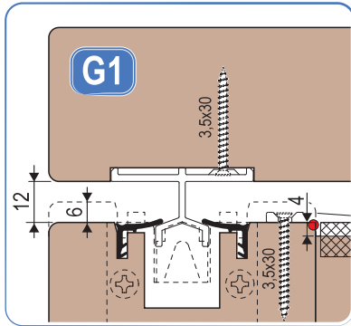
REDUCED UPPER GUIDE
